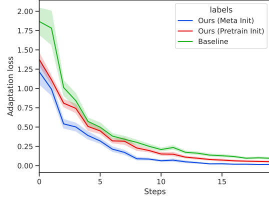
Figure 4: Analysis on prompt learning process.
